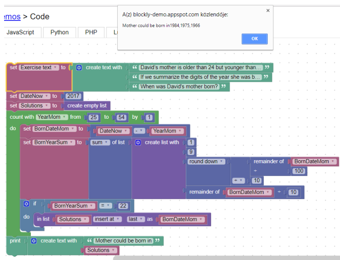
Figure 2 Blockly Code implementation of 'David's mother' task 1
