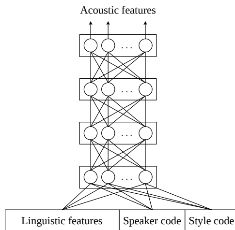
Figure 2 Auxiliary input model (AIM) of [20]
