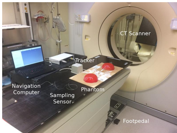
Figure 10 Experimental setup for electromagnetic reconstruction
