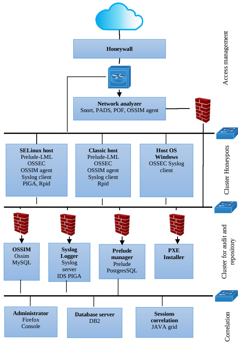
Figure 1: Clustered high-interaction honeypot architecture
