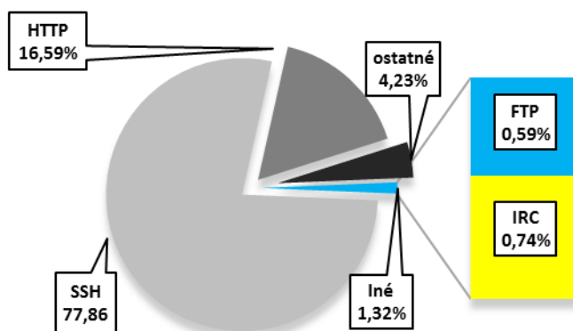
Figure 5 Generated alarms, by the respective ports
