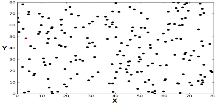
Figure 5 Random network
