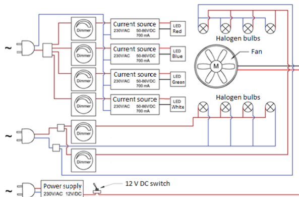
Figure 5 The power supply wiring of the sun simulator
