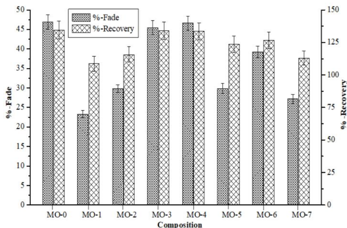
Figure 6 Variation of %-fade and %-recovery of the composites
