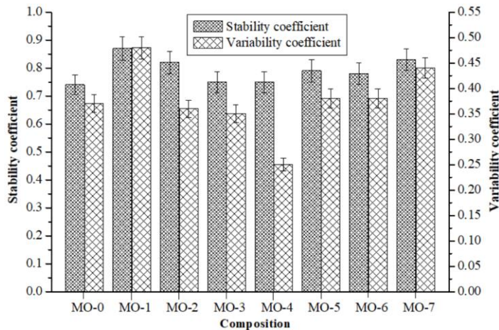
Figure 5 Stability and variability coefficients of the composites
