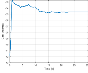
Figure 11 Coverage cost
