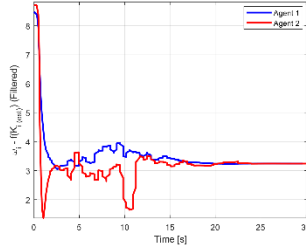
Figure 13 The value of w_i - f(\hat{R}_i)
