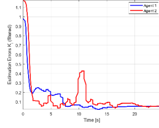
Figure 12 Estimation errors
