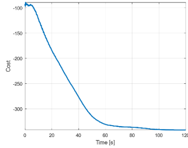
Figure 5 Coverage cost
