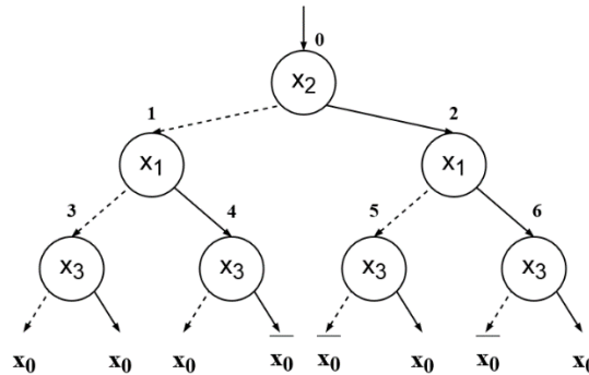
Figure 8 Unreduced RViBDD for f_2 from Example 2
