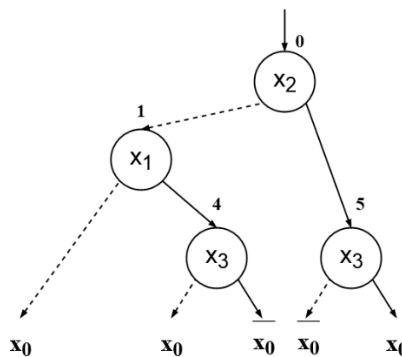
Figure 9 Reduced RViBDD for f_2 from Example 2
