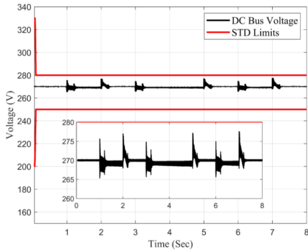
Figure 9 The 270 VDC bus voltage profile with EMA load
