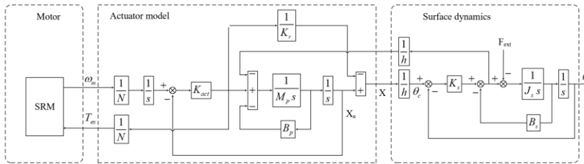
Figure 7 EMA simulation model
