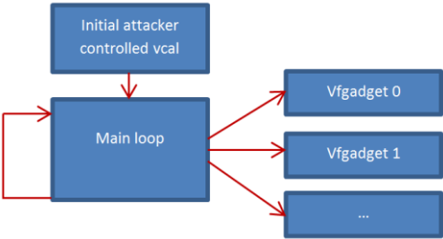
Figure 13 Counterfeit Object Oriented Programming [34]
