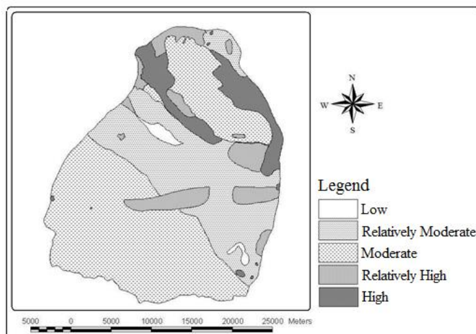
Figure 2 Zoning map of desertification intensity in Kheyr Abad
