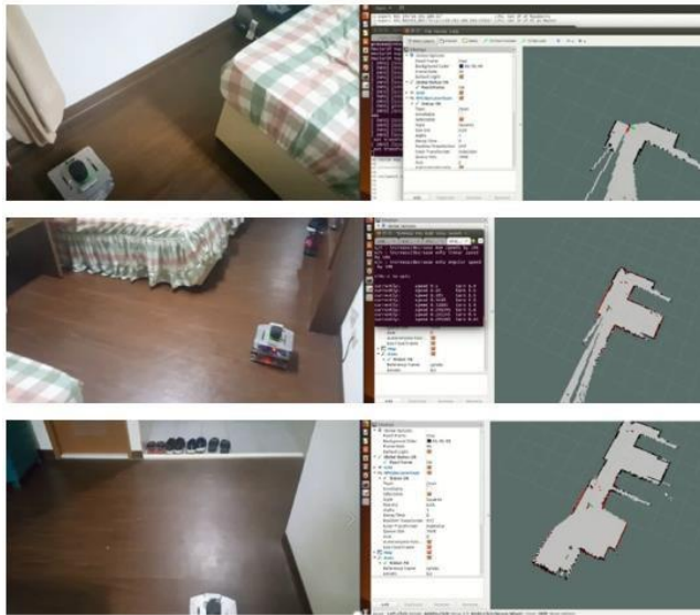
Figure 1 LiDAR-based SLAM results
