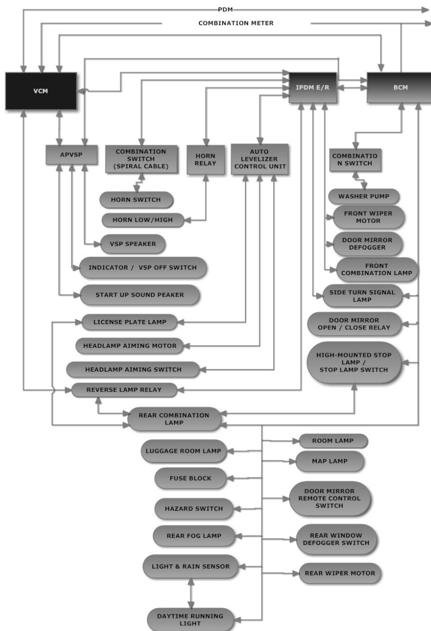
Figure 2 The electronic network of the Driver Control System
