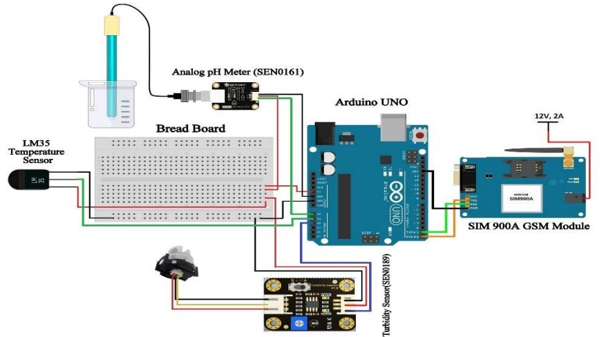
Figure 4 Hardware Simulation Process of Sensors
