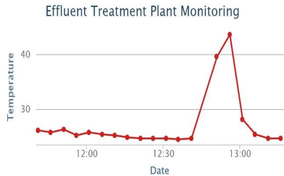
Figure 6 Temperature Data in Cloud
