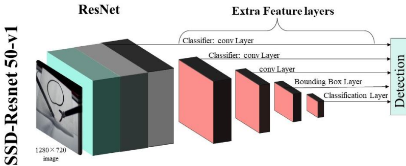
Figure 3 SSD-ResNet50 V1 FPN Architecture
