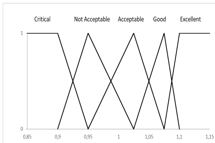
Figure 2 Fuzzy function (Source: Own edition)
