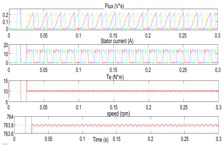
Figure 4 The motor performance of AFOSMC without uncertainties ( J=0.05 )
