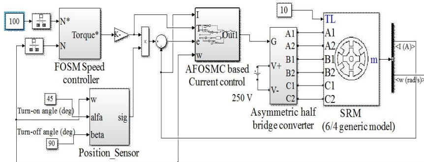
Figure 3 The MATLAB model of the proposed system
