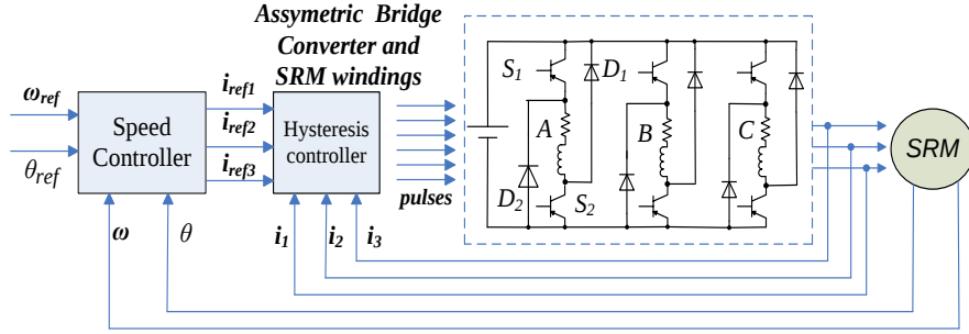
Figure 1 The Block Diagram of the Proposed System
