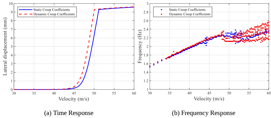
Figure 11 Comparison of bifurcation diagrams for lateral displacement, Axle Load = 18 kN
