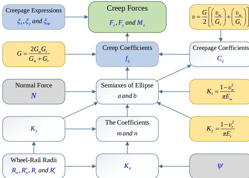
Figure 4 Creep forces flowchart
