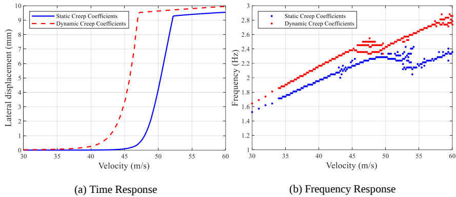
Figure 12 Comparison of bifurcation diagrams for lateral displacement, Axle Load = 120 kN
