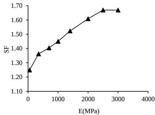
Figure 5 Geocell stiffness against SF for the ST2-30
