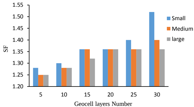
Figure 1 Effect geocell opening size on SF of ST2-30 embankment
