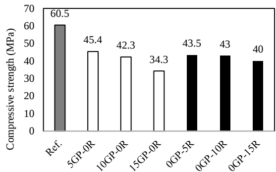
Figure 3 Compressive strength and flowability of concrete specimens
