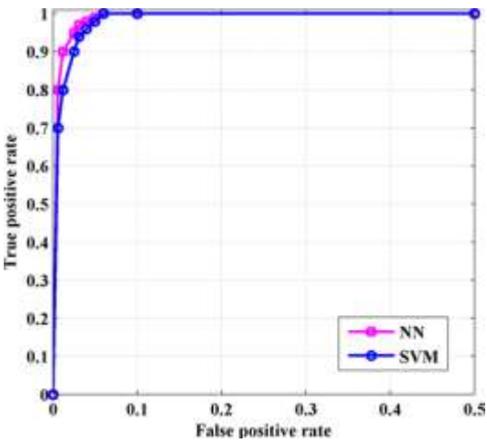
Figure 11 ROC curve for NN and SVM classifier
