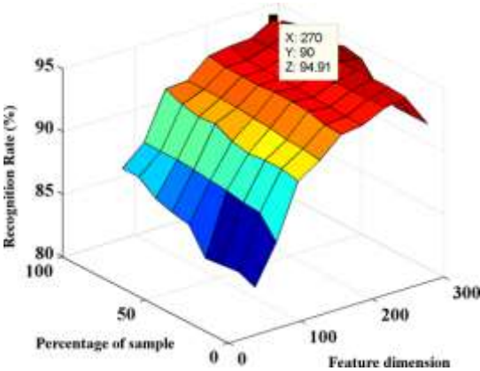
Figure 10 Recognition rate vs. Feature Dimension vs. PS (for AR, considering CRC_RLS)
