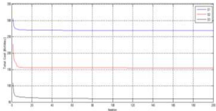
Figure 8 Convergence characteristics of CSOS for the operation scenarios
