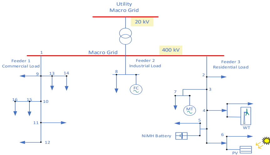
Figure 1 A typical low voltage microgrid [20]
