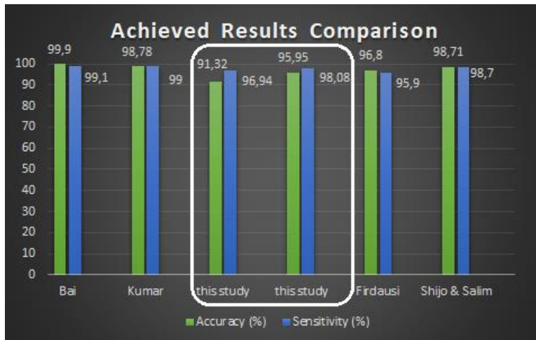
Figure 3 Comparison of the Best Algorithms from the Analysed Papers in Graph Form
