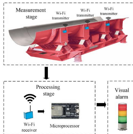
Figure 4 General scheme of the fault detection system
