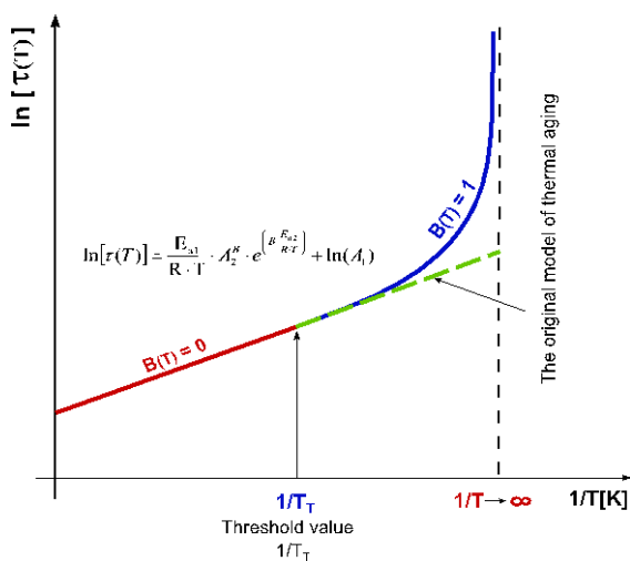
Figure 2 Thermal Aging Model Respecting the Threshold – threshold in the aging curve
