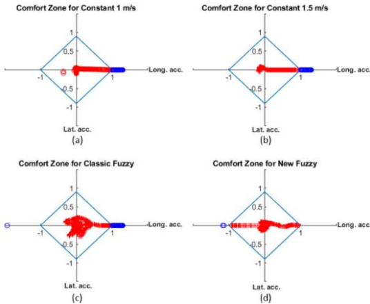
Figure 13 Comfort zone with longitudinal and lateral accelerations. (a) Constant 1 m/s. (b) Constant 1.5 m/s (c) Classic Fuzzy. (d) New Fuzzy
