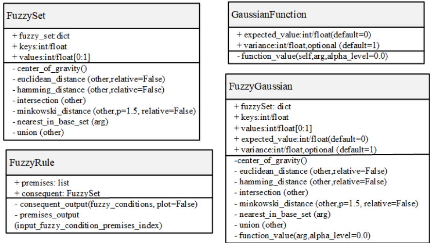
Figure 4 The main classes of the Loginf module
