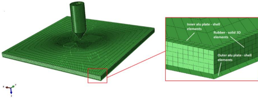
Figure 7 FE model of aluminium plates and rubber
