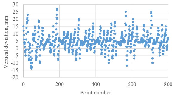
Figure 5 Registering track deviations in a vertical plane
