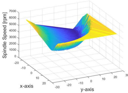
Figure 12 Required spindle speed
