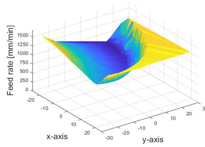
Figure 13 Required feed rate
