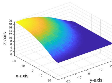
Figure 7 The tool position determined by reading the APT file
