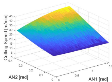
Figure 11 Cutting speed versus surface inclination
