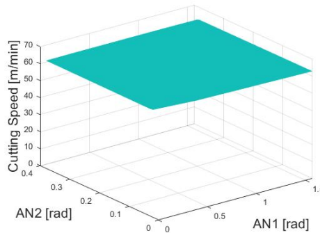
Figure 14 Theoretical cutting speed
