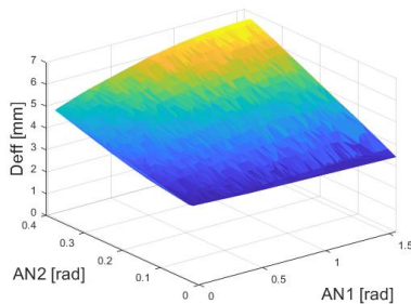
Figure 10 Working diameter versus surface inclination
