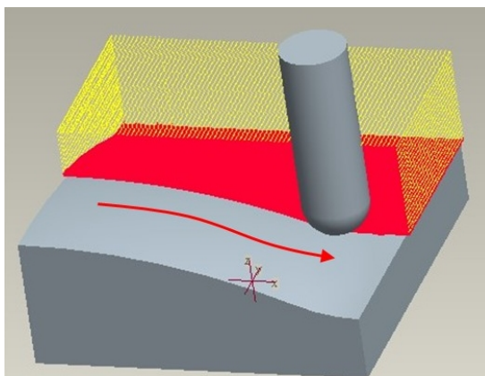
Figure 5 Down milling process in CAM simulation
