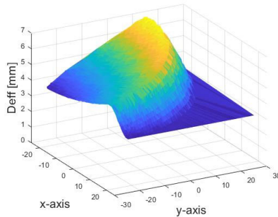
Figure 8 The working diameter
