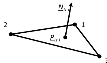
Figure 1 Definition of a triangle in the STL language
