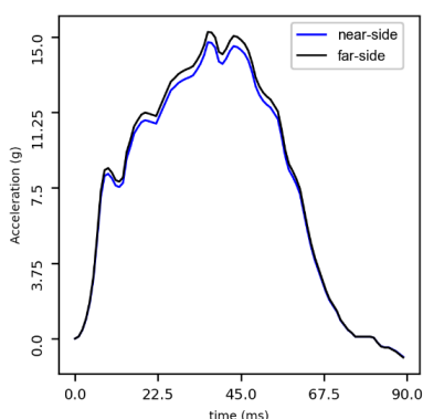
Figure 5 Acceleration pulse
