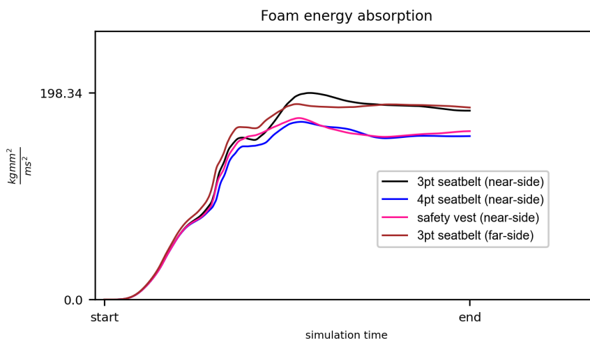
Figure 19 Seat energy absorption
