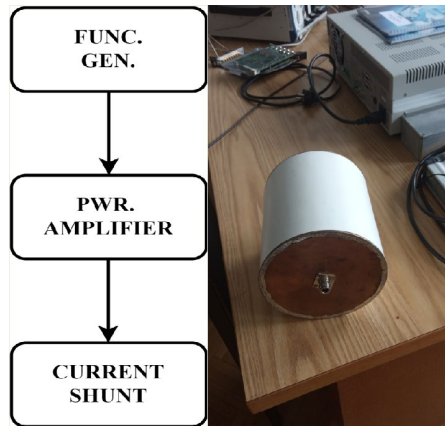
Figure 7 Measurement scheme and tested current shunt
