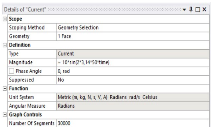
Figure 9 Settings for alternating current in the ANSYS application
