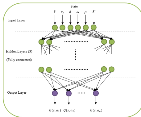
Figure 5 The reinforcement DQN structure
