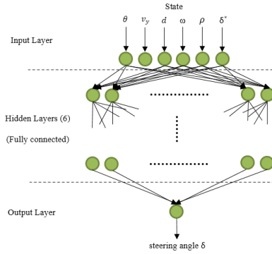
Figure 4 The DNN model structure
