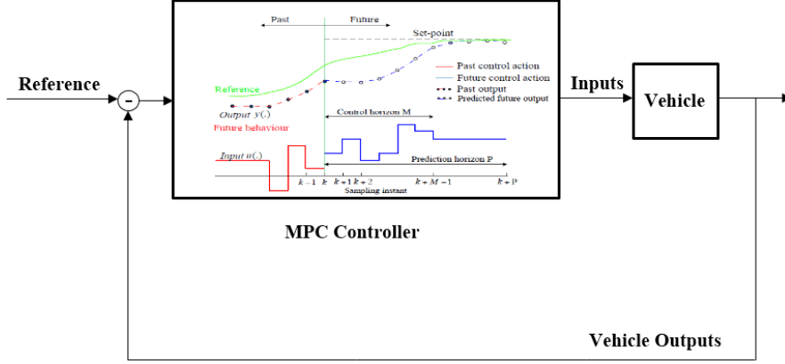
Figure 3 MPC controller design
