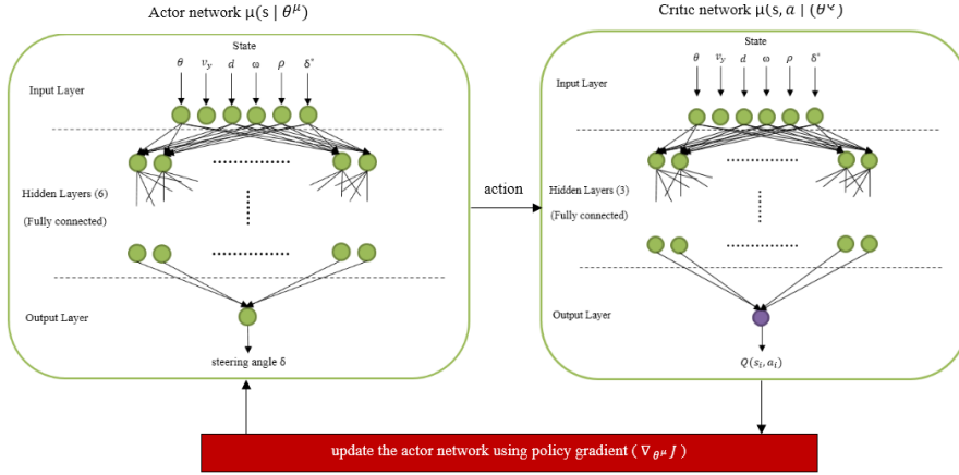
Figure 6 The structure of the actor-critic networks - combined model
