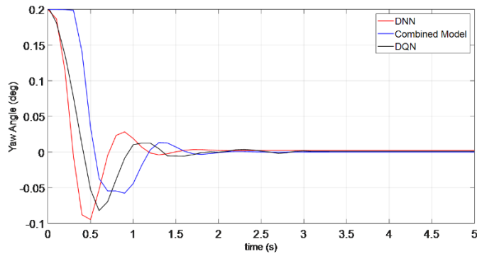
Figure 12 Vehicle response to the control actions of the DNN, DQN - yaw angle
