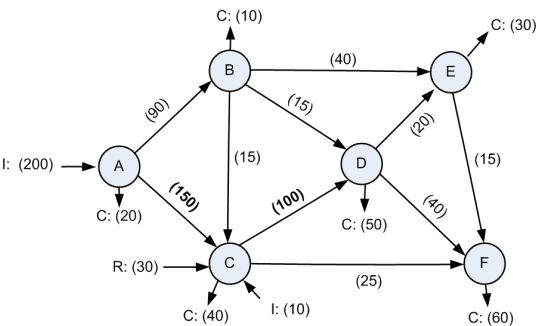
Figure 3 The simple example network with extended capacities. Modified values are emphasized with bold typeface.
