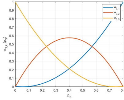
Figure 4 CNO type weighting functions of TP model 3
