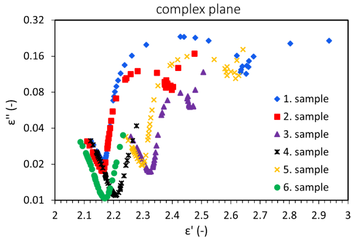
Figure 4 Complex permittivity in the complex plane \varepsilon''=f(\varepsilon')
