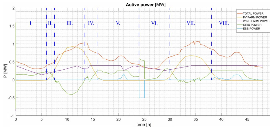
Figure 7 Characteristics of active powers
