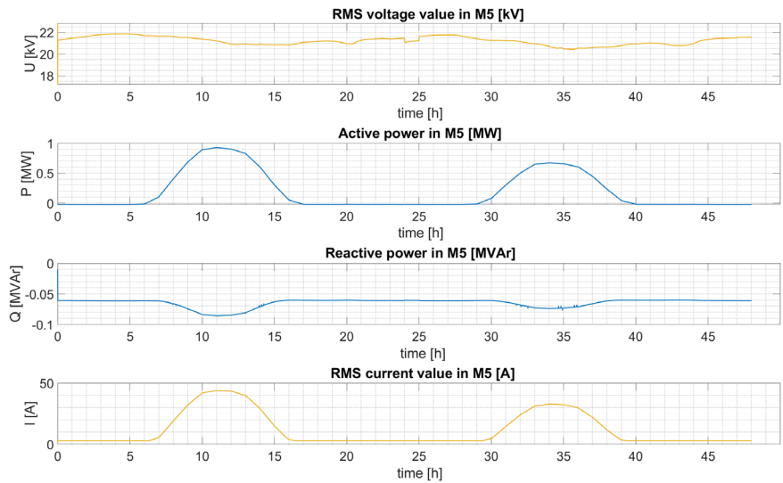
Figure 13 Electrical parameters that were measured at the M5 node
