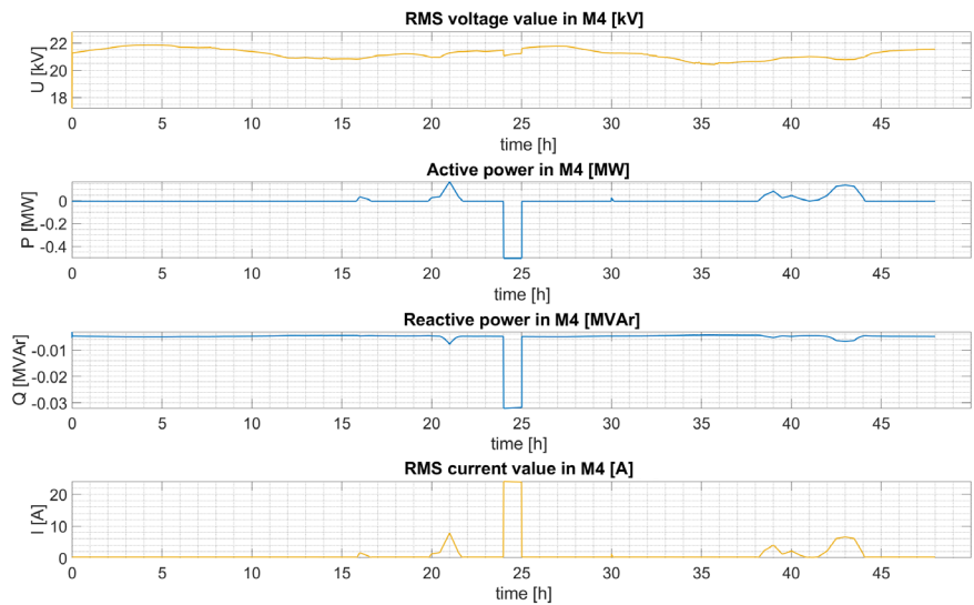
Figure 12 Electrical parameters that were measured at the M4 node
