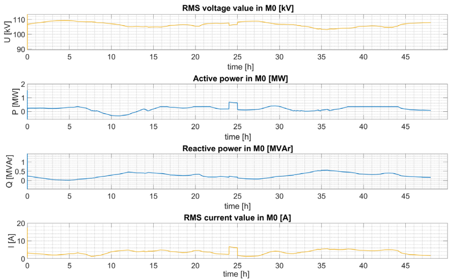
Figure 8 Electrical parameters that were measured at the M0 node
