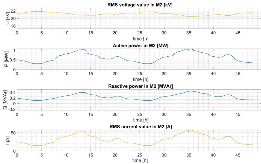
Figure 10 Electrical parameters that were measured at the M2 node
