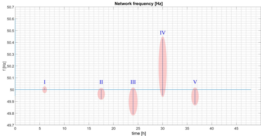
Figure 15 The network's frequency fluctuation throughout the measured period
