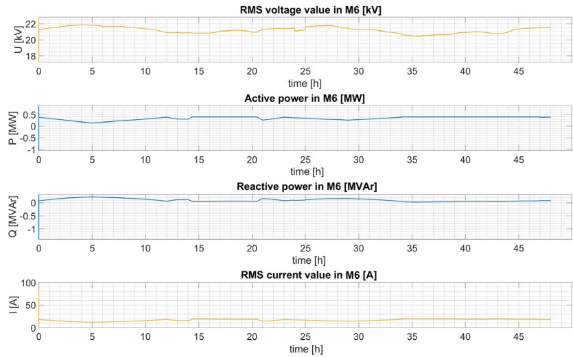
Figure 14 Electrical parameters that were measured at the M6 node
