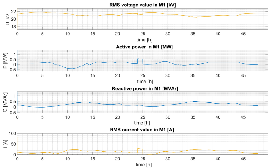
Figure 9 Electrical parameters that were measured at the M1 node
