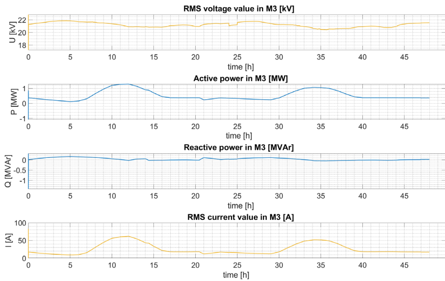
Figure 11 Electrical parameters that were measured at the M3 node
