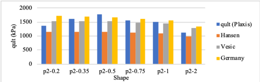
Figure 12 Comparison of Plaxis' calculation of bearing capacity and empirical equations of bearing capacity for a 50-m² area of plus foundation
