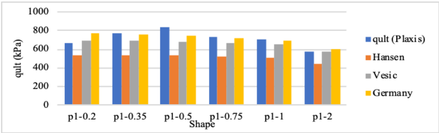
Figure 11 Comparison of Plaxis' calculation of bearing capacity and an empirical equations of bearing capacity for a 9-m² area of plus foundation
