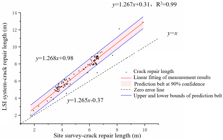
Figure 8 Regression analysis of circumferential crack length
