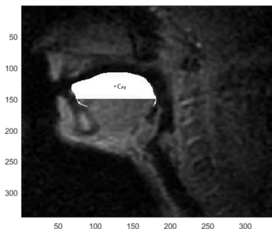
Figure 8 The centroid of sound /ε/
