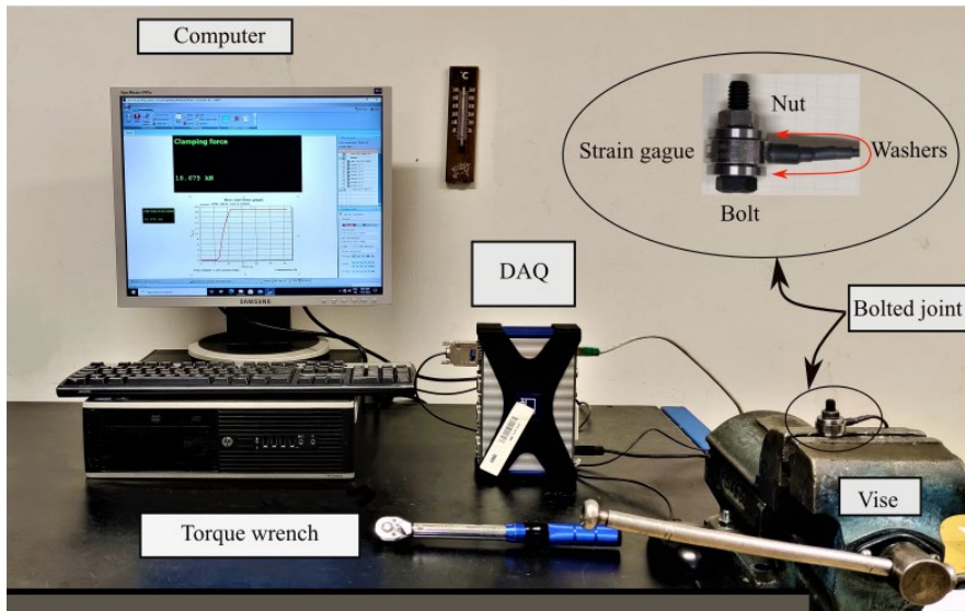
Figure 6 Experimental setup
