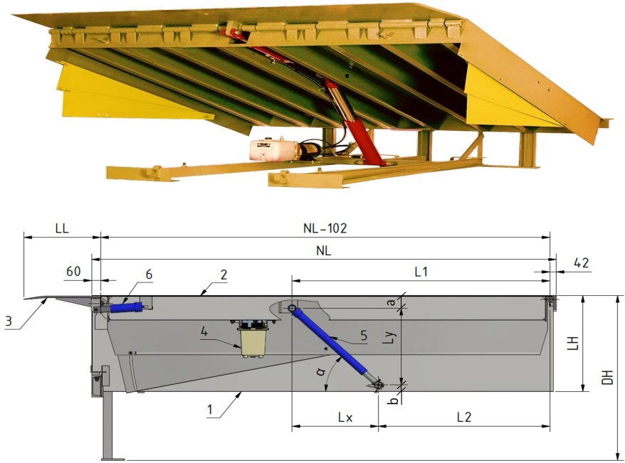
Figure 4 Constructive parameters of the lifting system designed for the Autodock docking leveler
