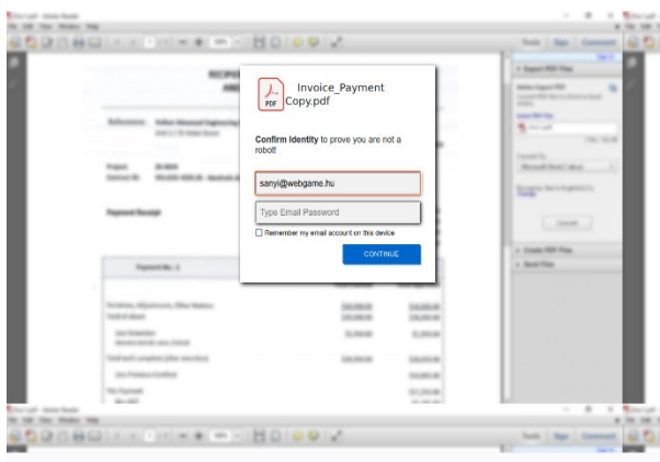
Figure 3 Phishing form
