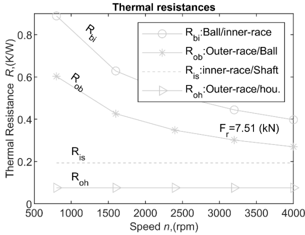
Figure 6 Thermal resistances R_i (K/W)
