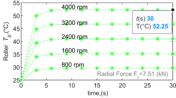
Figure 8 Temperature distribution of the balls T_b
