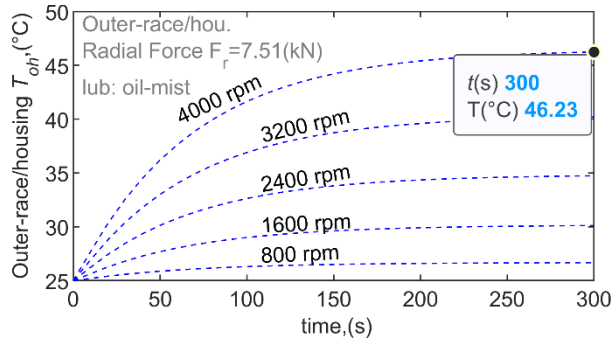
Figure 9 Temperature distribution of the outer-race/ housing T_{oh}
