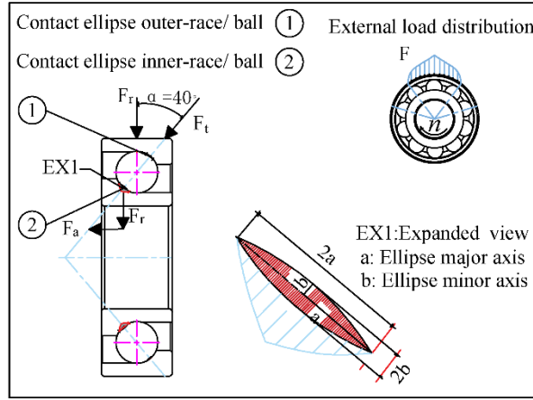
Figure 2 Force distribution and contact region (Source: Author)
