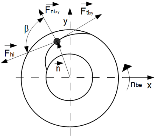
Figure 3 Forces acting on a ball moving in track in the x-y
