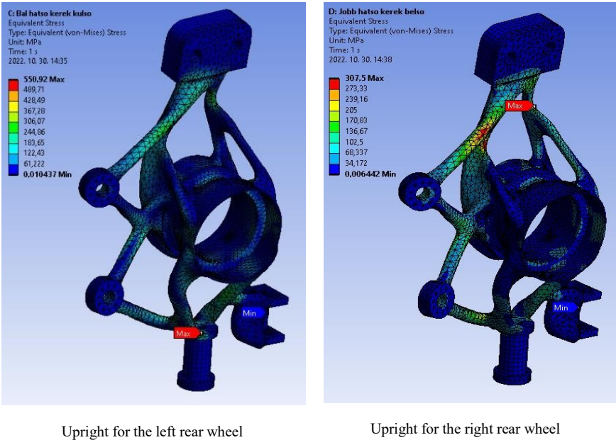
Figure 4 The Von Mises stress distribution of an upright designed with shape optimization while presenting deformation
