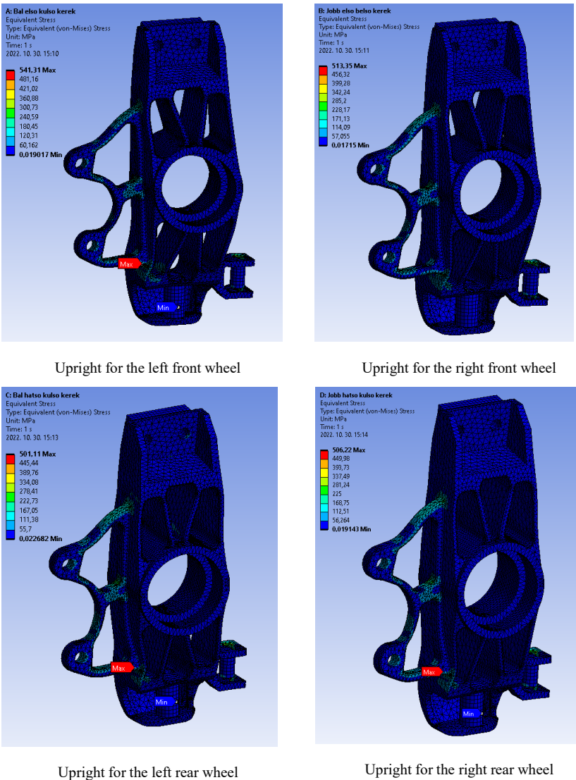
Figure 3 The Von Mises stress distribution of an initial upright designed ANSYS
