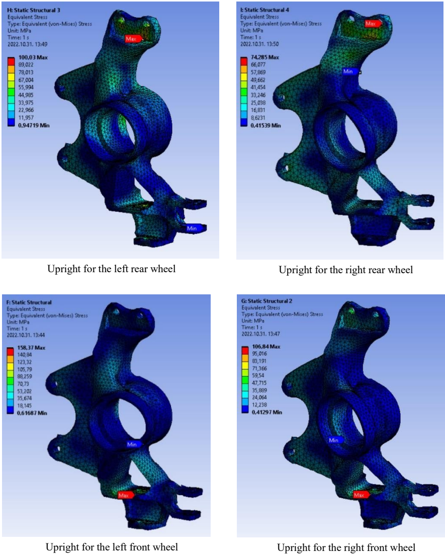
Figure 5 The Von Mises stress distribution of an upright designed with shape optimization while presenting deformation
