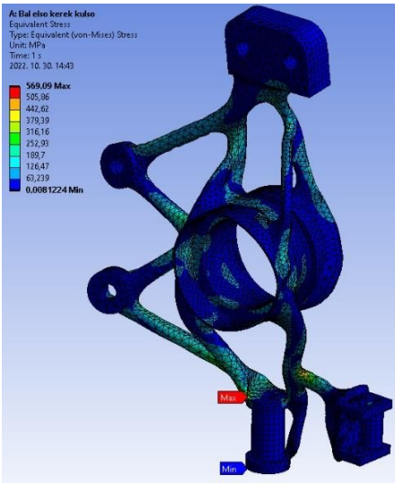
Upright for the left front wheel
