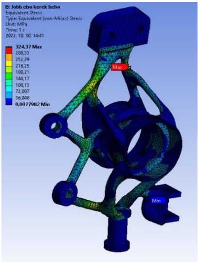
Upright for the right front wheel
