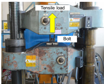
(a) Calibration test setup
