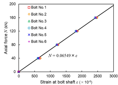
(b) Relationship between axial force and strain
