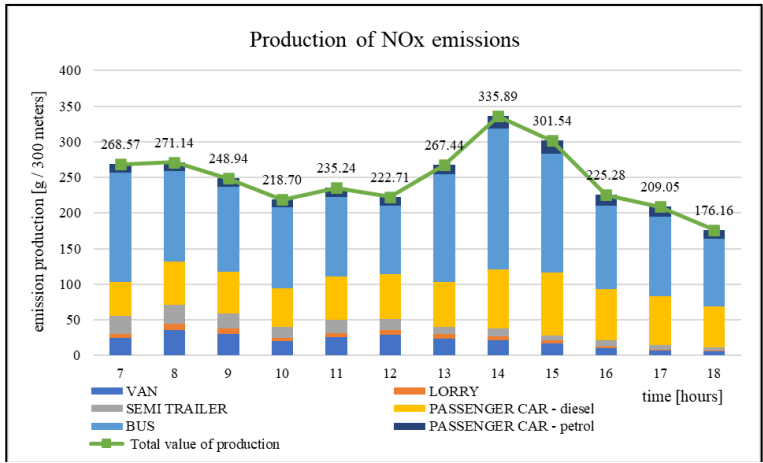
Figure 6 Production of NO x emissions in the monitored section [authors]
