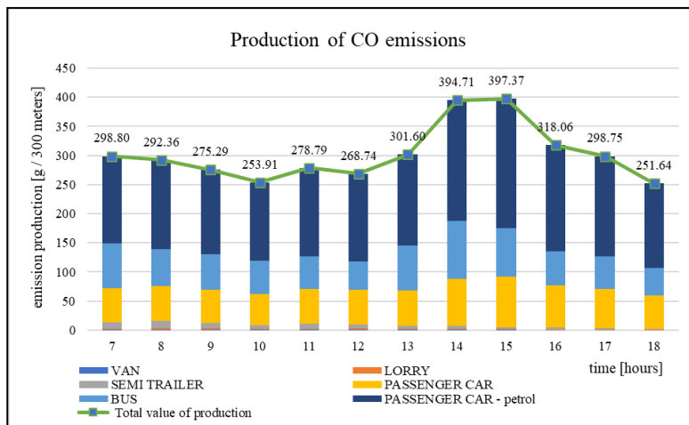
Figure 4 Production of CO emissions in the monitored section [authors]
