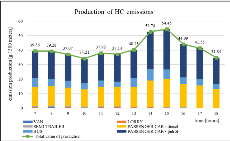
Figure 5 Production of HC emissions in the monitored section [authors]
