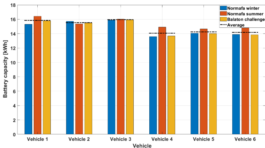
Figure 6 Calculated battery capacities from measurements
